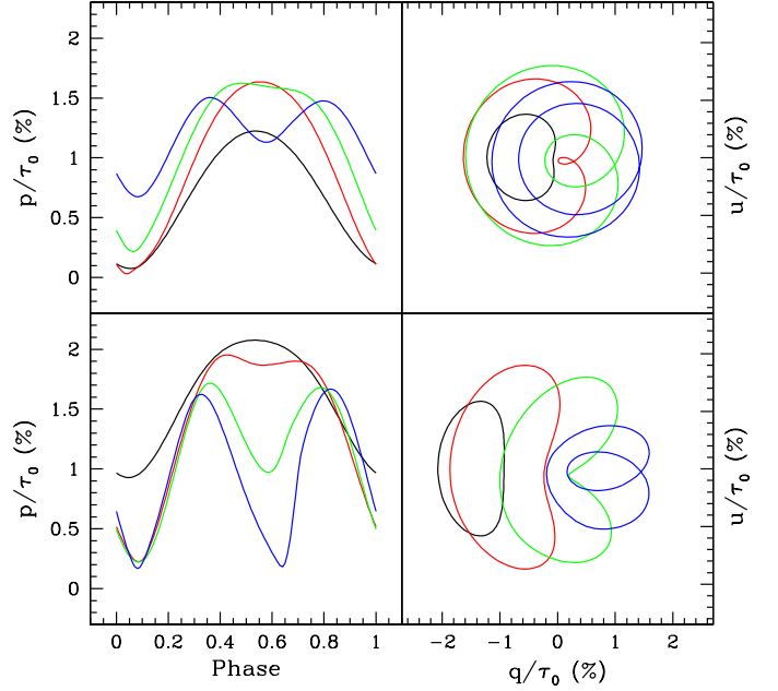
Fig. 6. Periodic variations in polarization are shown here for CIRs that emerge from different latitudes of the star. The layout of the figure is the same as in Fig. 5. Here the colors are for CIRs at latitudes of \vartheta = 20^\circ (black), 40^\circ (red), 60^\circ (green), and 80^\circ (blue).
