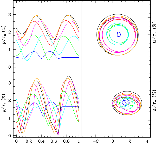
Fig. 5. Periodic variable polarization for two equatorial CIRs. The format is the same as in Fig. 4 with light curves to the left, q - u plane variations to the right, a viewing perspective of i = 30^\circ at the top, and i = 60^\circ along the bottom. The two CIRs are shifted from each other by an angle \Delta\varphi of 0^\circ (black), 30^\circ (red), 60^\circ (green), 90^\circ (dark blue), 120^\circ (light blue), 150^\circ (magenta), and 180^\circ (orange).
