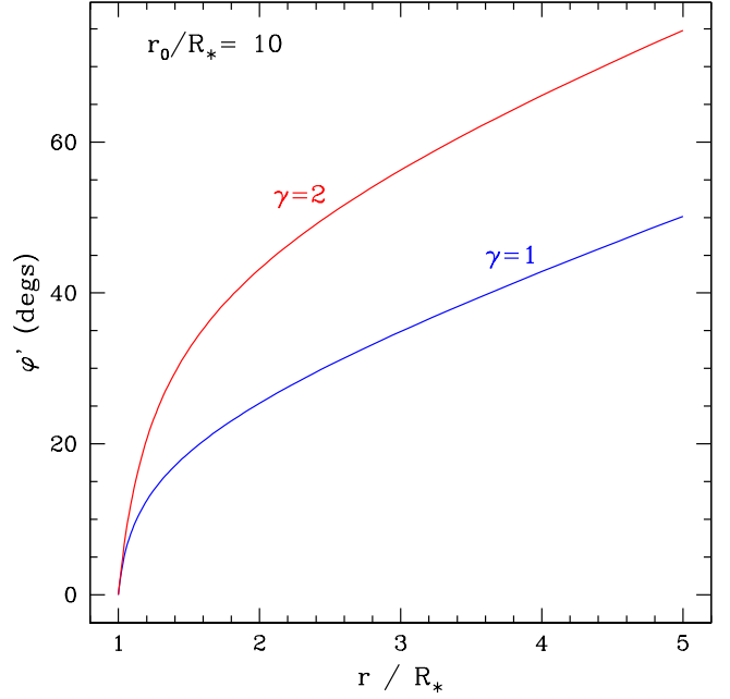
Fig. A.1. Comparison of the azimuth location of the CIR centroid with radius from the star. Here blue is for \gamma = 1 , and red is for \gamma = 2 . This example uses a wind radius of r_0 = 10R_* . The value of \phi' is generally between 50% to 100% larger for \gamma = 2 than for \gamma = 1 indicating that a spiral CIR is considerably more curved at a given radius for the higher \gamma case.
