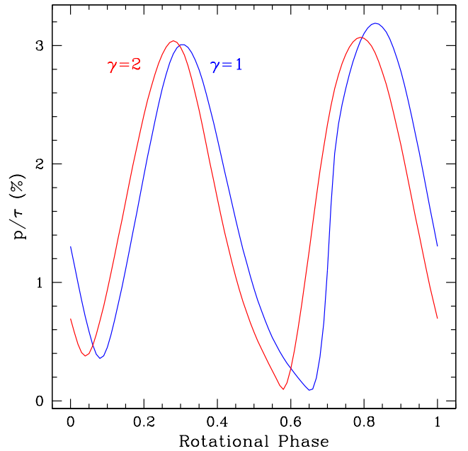
Fig. A.2. Comparison of polarization light curves for the \gamma = 1 and \gamma = 2 cases shown in the previous figure. The polarization is plotted as normalized to the wind optical depth along a radial. The case of \gamma = 1 produces a relatively stronger polarization signal (per unit optical depth) than in the case of \gamma = 2 . The polarization extrema are slightly shifted in phase between the two cases.
