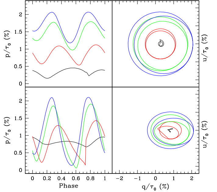
Fig. 4. Periodic variations of polarization with stellar rotational phase for CIRs with different winding radius values. Left panels are for polarization light curves with phase; right panels are for variations in the q - u plane. Top panels are for a viewing inclination of i = 30^\circ and lower for i = 60^\circ . Different curves are for different winding radii, with values r_0/R_* = 1 (black), 3 (red), 9 (green), and 27 (blue).
