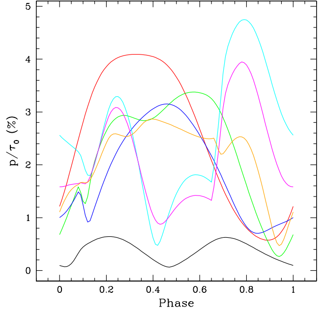
Fig. 7. Periodic polarization light curves for a randomized distribution of CIRs across the star. Each curve represents the addition of one more randomly placed CIR. The curves correspond to a number of CIRs of 1 (black), 2 (red), 3 (green), 4 (dark blue), 5 (light blue), 6 (magenta), and 7 (orange). Table 1 lists model parameters of the individual CIRs.
