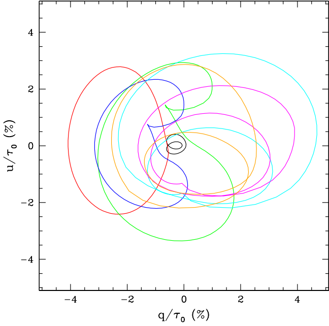
Fig. 8. Polarization model results from Fig. 7 displayed in the q - u plane. The colors correspond to the identifications indicated in Fig. 7.
