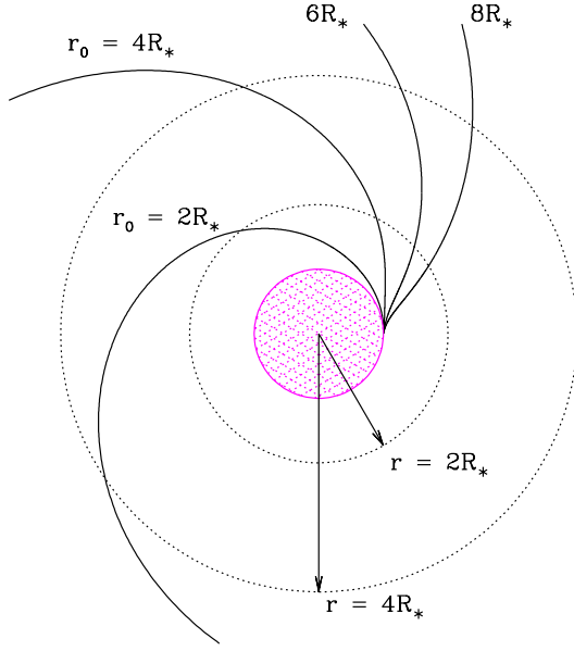
Fig. 3. Examples of the spiral shape for the CIRs as a function of the winding radius, r_0 . The figure displays the centroid of four different CIRs with distance from the star. The star is the shaded magenta circle. The CIRs are in the equatorial plane, shown here as seen from above. The two larger dotted circles are reference circles at 2R_* and 4R_* . The different spirals are distinguished by different winding radii as labeled. Lower values of r_0 place the transition from a cone-shaped CIR to a spiral one closer to the star; higher values of r_0 indicate that the CIR has small curvature until achieving large distances from the star.
