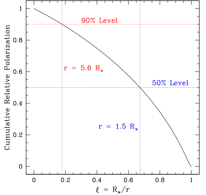
Fig. 2. Plot of the normalized cumulative polarization in terms of distance from the star. The figure applies when the polarization calculation is separable (see text). In the case \gamma = 1 , reference lines show that half of the polarization will be determined within half a stellar radius above the atmosphere; 90% will be determined between one and 5.6 stellar radii.
