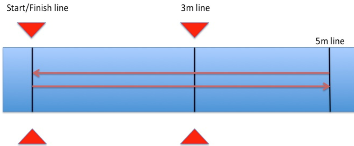
Figure 1: Schematic approach of pre-planned COD test
