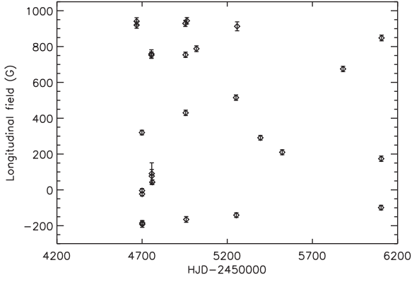
(a) Longitudinal field versus HJD
