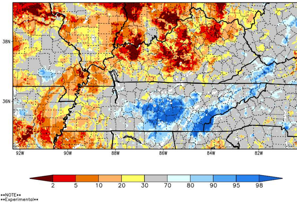
SPoRT-LIS 0-200 cm Soil Moisture percentile valid 31 Aug 2023
