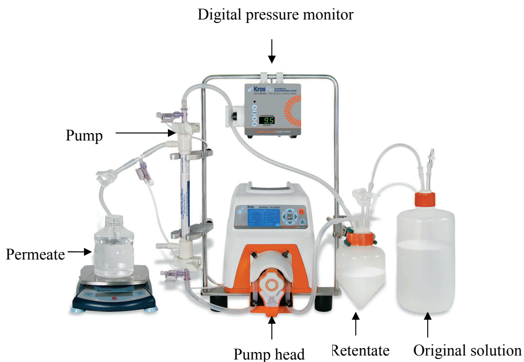
Figure 8 Diagram of Kross flow research Ili TFF system (Source: NICOMP 380 ZLS zeta sizer, 2010)
