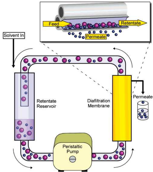
Figure 9 Schematic representation of the flow path of the Krossflow system.
