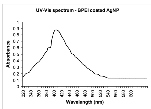
Figure 3 UV-Vis spectra of the selected types of AgNPs
